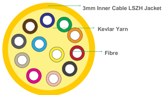
12 Fibre SM 3mm Trunk Cable
