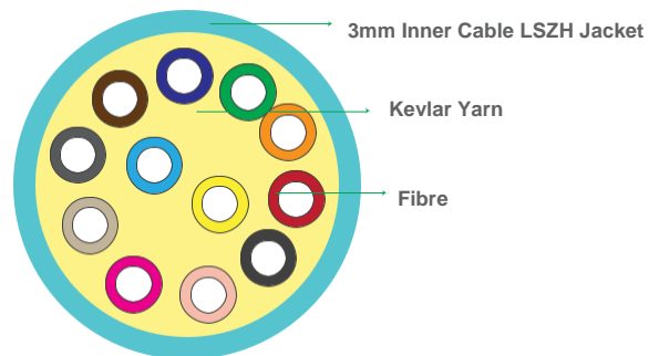
12 Fibre OM3/OM4 3mm Trunk Cable
